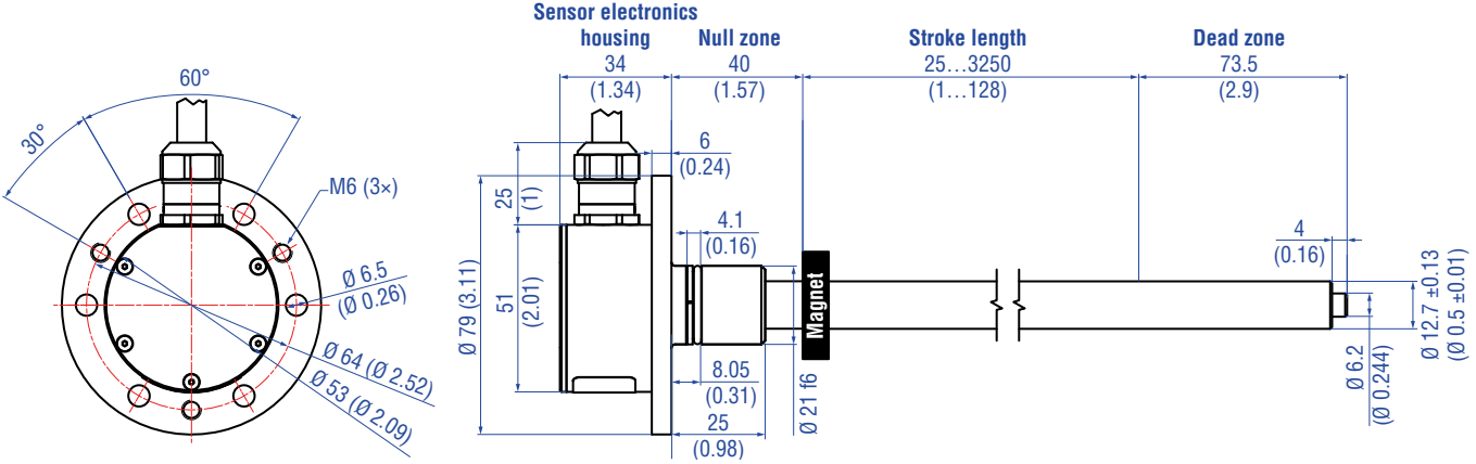
Controlling design dimensions are in millimeters and measurements in ( ) are in inches Fig. 2: Temposonics® GB-N / GB-S / GB-K / GB-J with ring magnet
