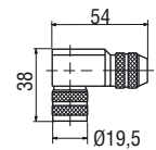
6 pin 90° female connector M16 Part No. 560 778
