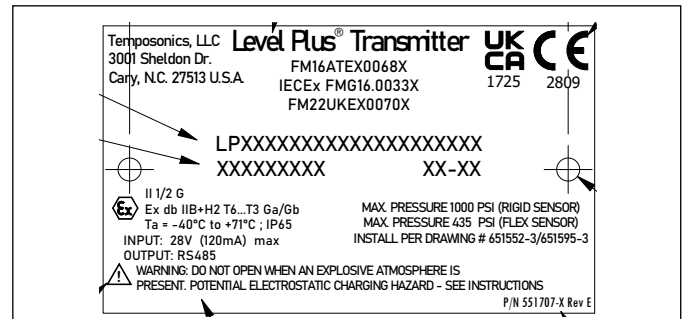
Fig. 58: Flameproof, ATEX/IECEX and UKCA label, Modbus or DDA Housing Option D, E, G, H, or L
