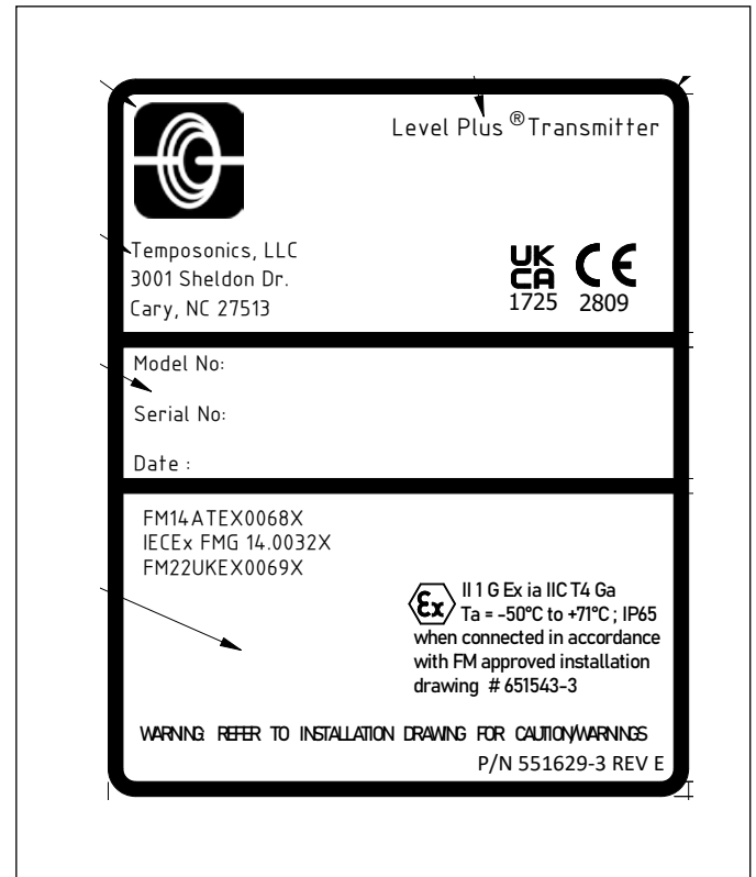
Fig. 50: Intrinsic Safe ATEX, IECEX, and UKCA label, Modbus and DDA, NEMA Housing
