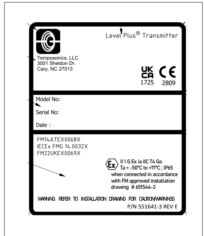
Fig. 51: Intrinsic Safe ATEX, IECEX, and UKCA label, Modbus and DDA, NEMA Housing
