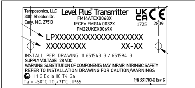
Fig. 52: Intrinsically Safe ATEX, IECEx, and UKCA label, Modbus and DDA, Single and Dual Cavity Housing
