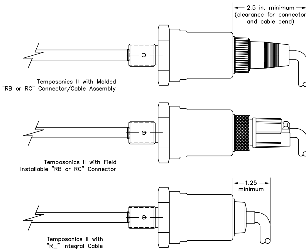
Temposonics II Connector/Cable Clearance Requirements
