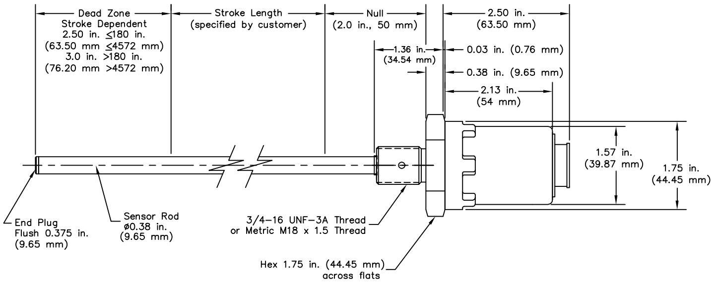
Temposonics II Dimension
