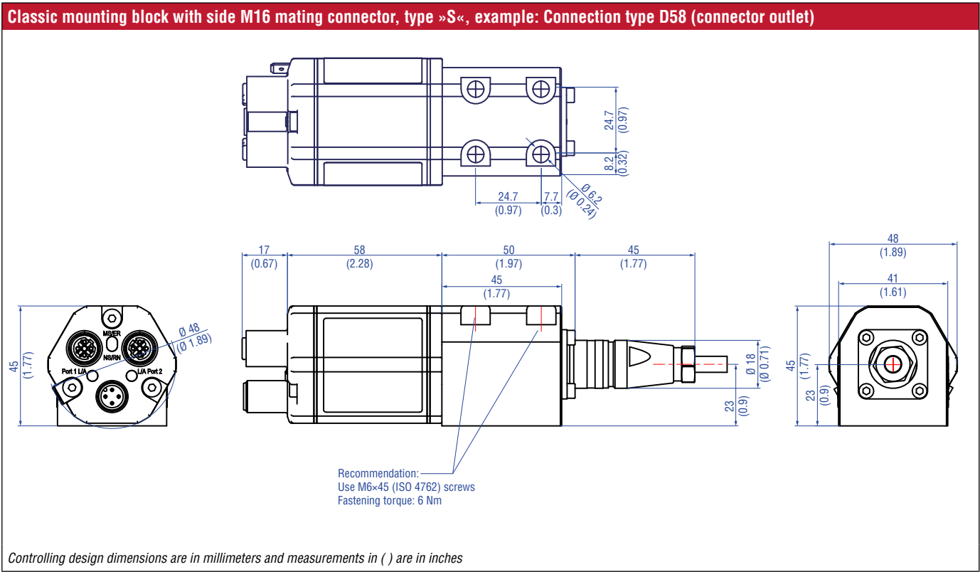
Fig. 4: Temposonics® RD5 sensor electronics & mounting block
